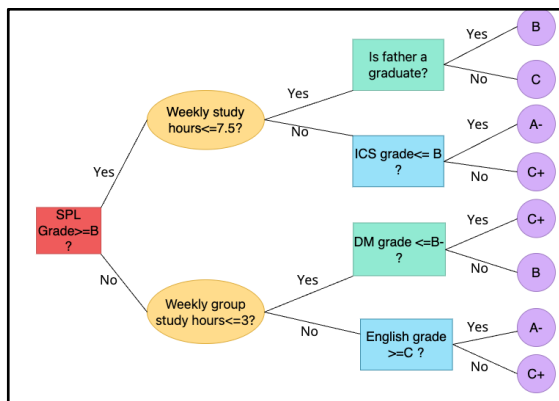
Figure 2. Decision Tree with academics
